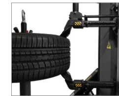
Double roller bead breakers.
